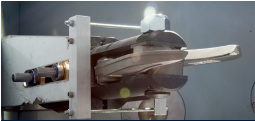
Hydraulic shear mounted on linear track and deployed by tong manipulators
